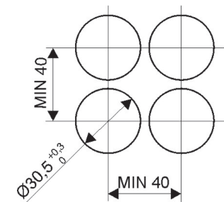
MOUNTING DIMENSIONS WITHOUT PANEL
