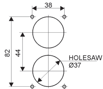
MOUNTING DIMENSIONS WITH SELÉN PANEL 540-462-01
