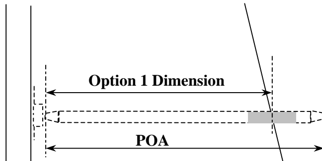
Option 1 - Wrap position optimised for pole contact with forestay
